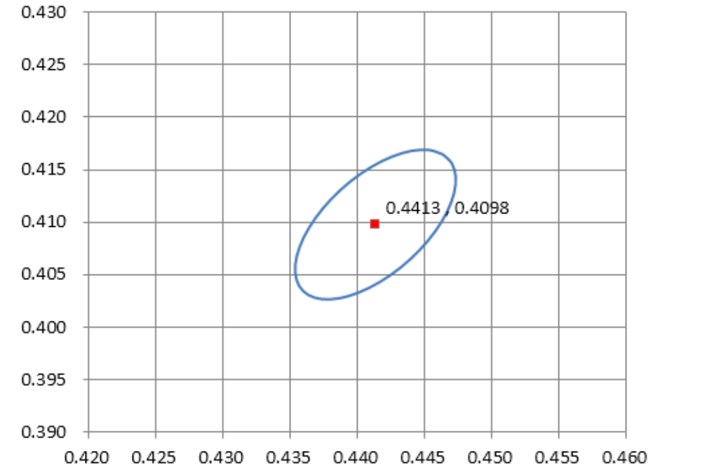
Chromaticity Bins: 1931 CIE Curve
